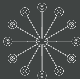
Art. 1710/CH12/KR/RS/V1 H 90 cm ø 120 cm Pø 14 cm 12 x E14 x 40W
