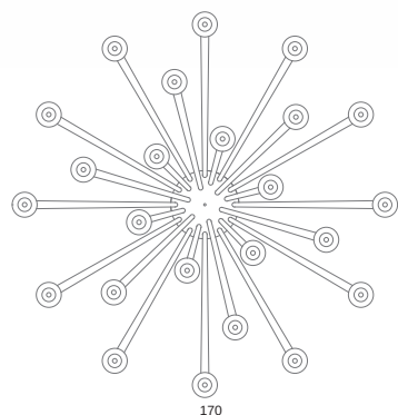
Art.1761 CH24 Ø 170 H 215 cm Pø 14cm 24x E14 x 40W
