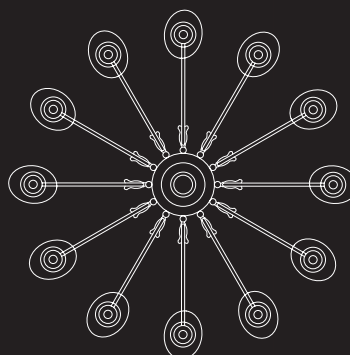
ART. 1774/CH12/ V1 H 66 cm ø 110 cm Pø 14 cm 12 x E14 x 40W
